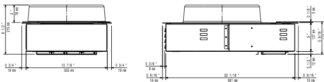
Side
